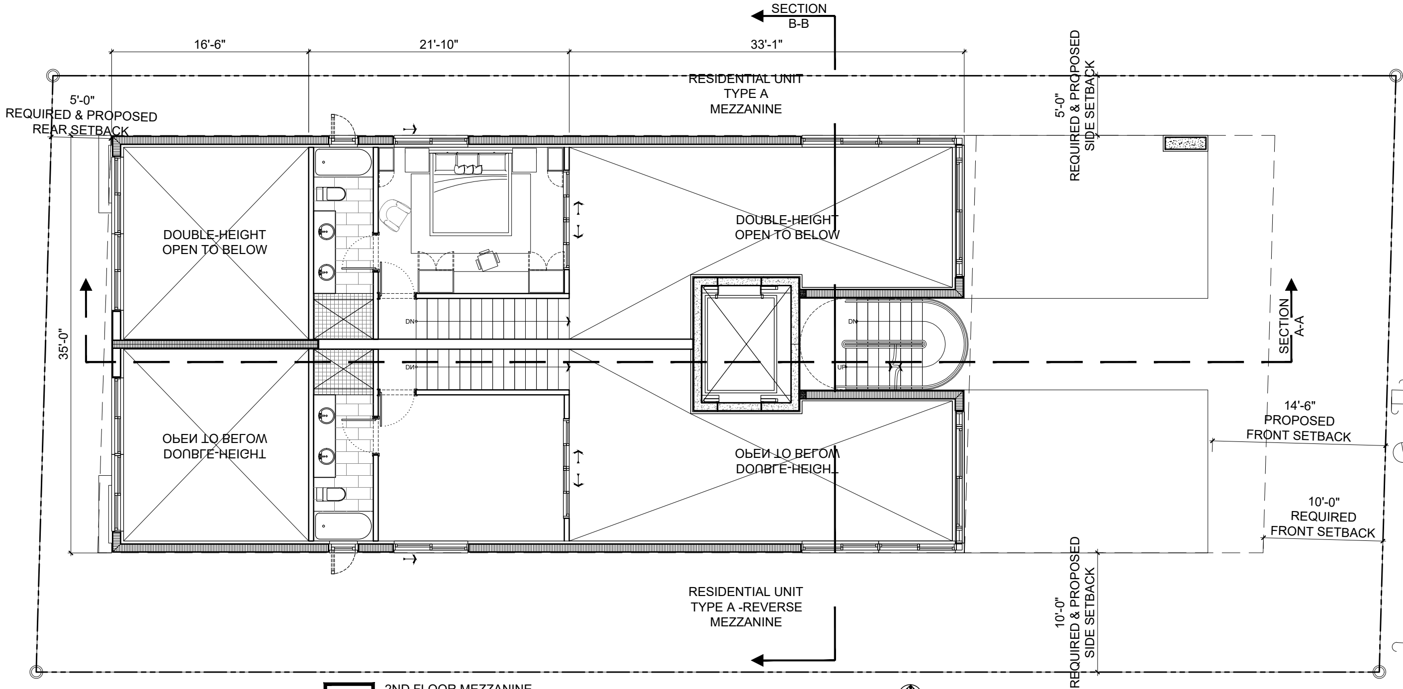
1 2ND FLOOR MEZZANINE SCALE: 1/8" = 1'-0"
